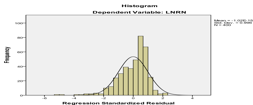
Figure 2: Normality of model errors
